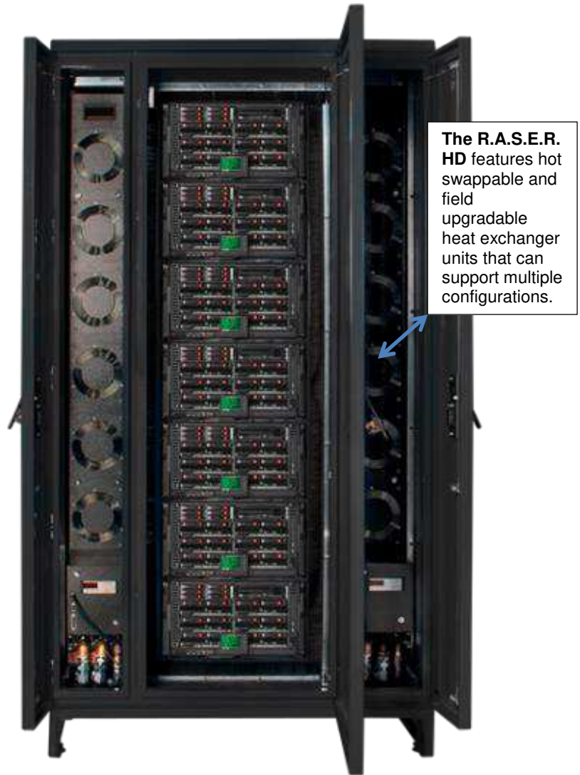
R.A.S.E.R. HD populated with *56 blade servers for a 40 kW solution.
